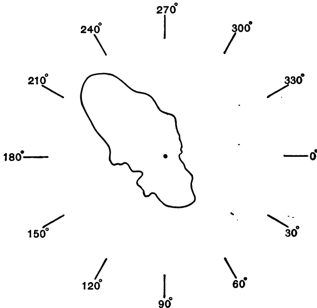
FIG. 6.—Observed Distribution of Proper Motions. (Groombridge Catalogue—R.A. 14^h to 18^h , Dec. +38^\circ to +70^\circ .)
